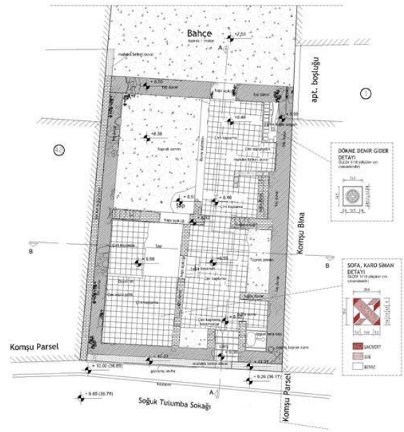
+2.00 KOTU (BODRUM) PLANI MALZEME ANALİZİ
